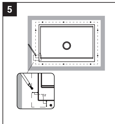
Clip's screw mounting holes should be 1/2" from edge of sink.
